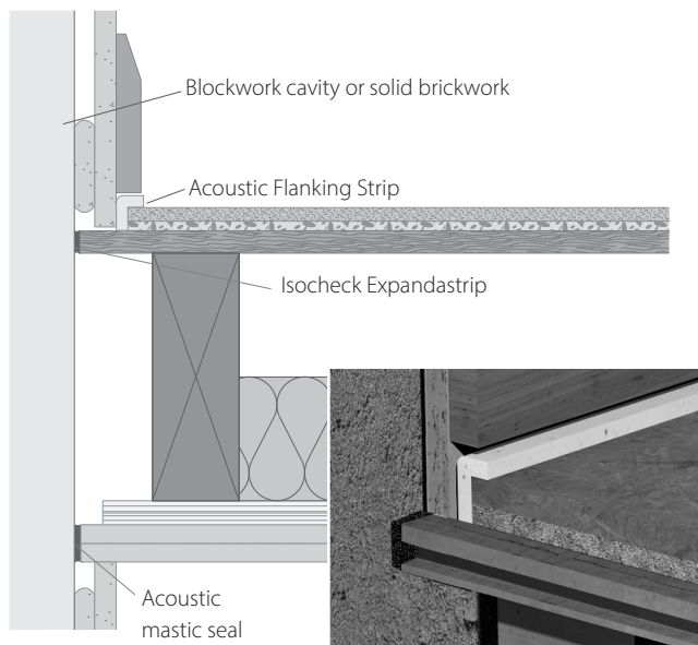
Flanking Strip turned back under skirting and trimmed flush with a sharp knife.
